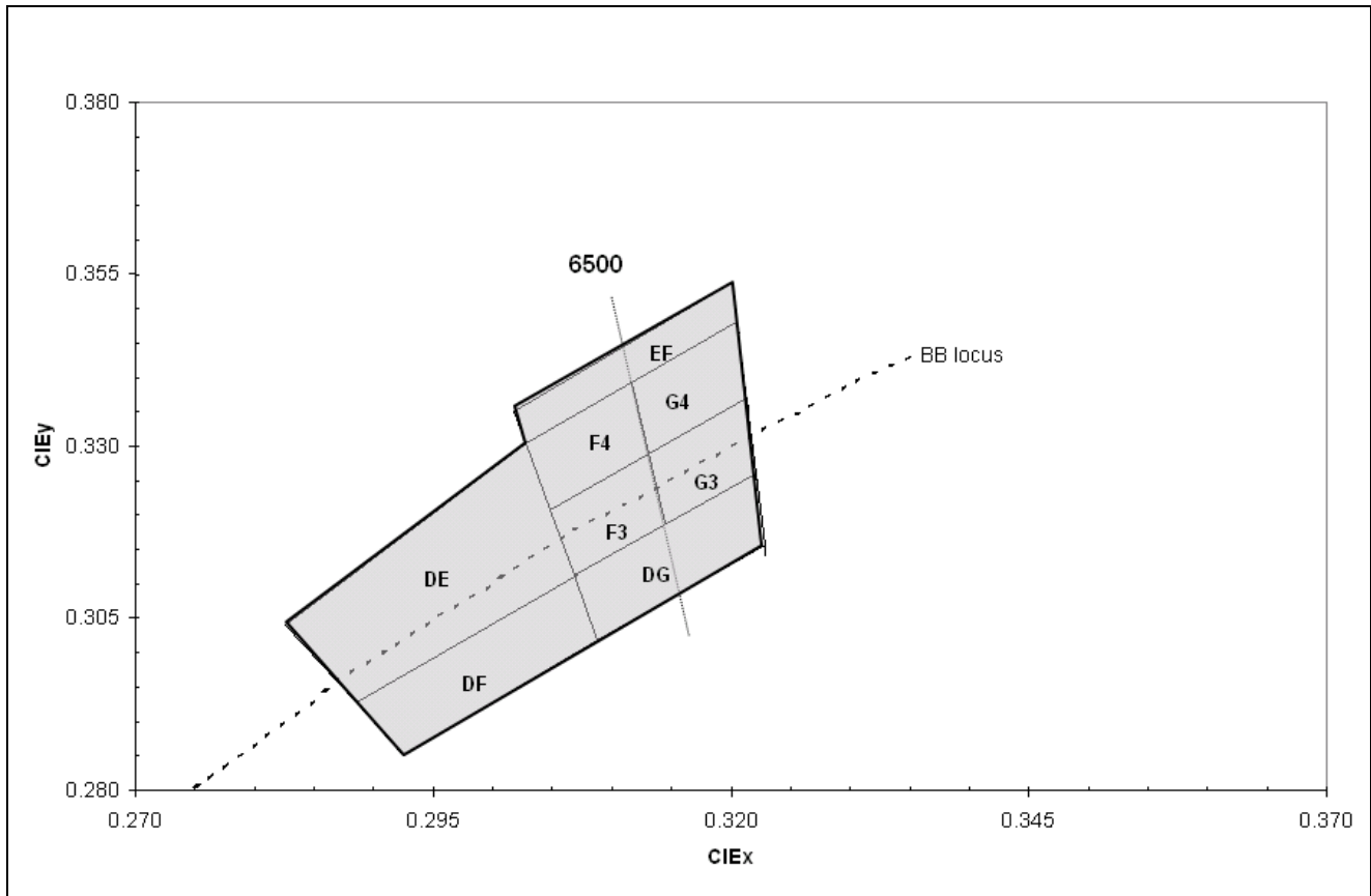
Luminus' Standard Chromaticity Bins: 1931 CIE Curve
